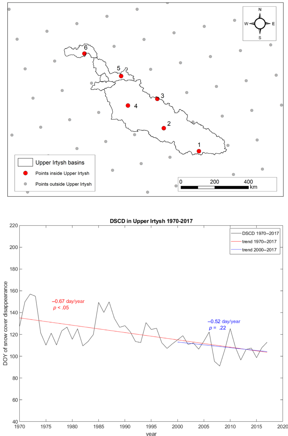
FIGURE 10 Location of grid cells from the NOAA CDR Northern hemisphere snow cover data set within the study area (top) and snow cover disappearance in Upper Irtysh from 1970 to 2017 (average of six pixels, bottom). CDR, Climate Data Record; NOAA, National Oceanic and Atmospheric Administration
