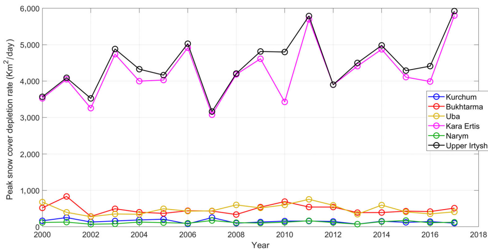
FIGURE 5 Peak snow cover depletion rate (PSCDR, \text{km}^2/\text{day} ) for each basin and the whole Upper Irtysh between 2000 and 2017
