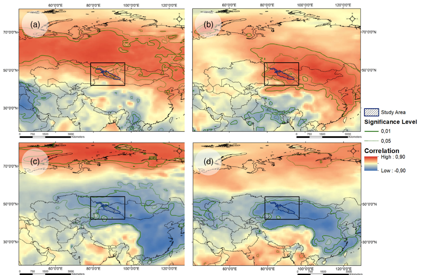
FIGURE 6 Correlation between winter/spring atmospheric circulation indices and temperature anomalies across Asia between 2000 and 2017. (a) Winter Arctic Oscillation (AO) – winter temperatures; (b) winter AO – spring temperatures; (c) winter Siberian High (SH) – winter temperatures; (d) spring SH – spring temperatures. The blue polygon inside the black box represents the location of the study area
